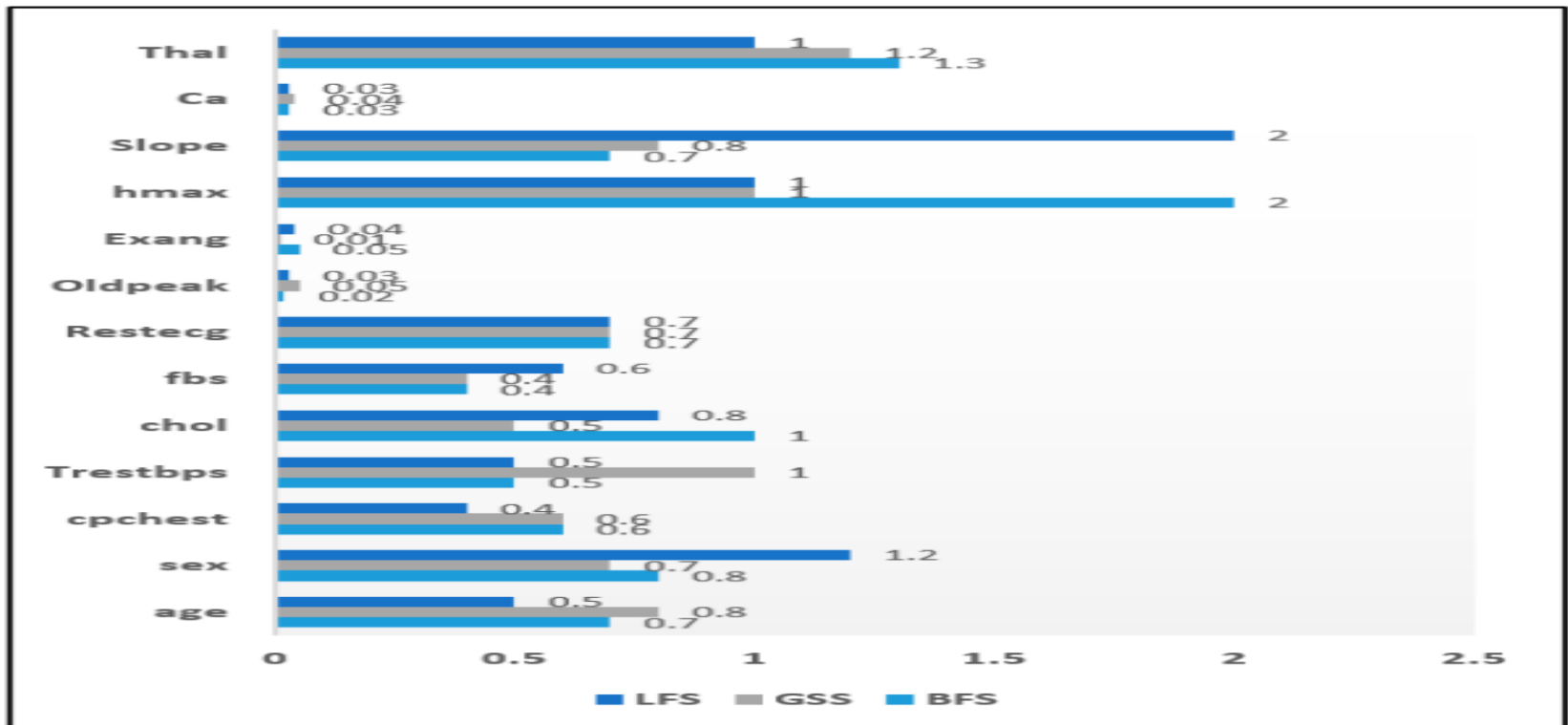
Figure 9. Attribute Significance Graph for the Heart disease dataset with Wrappers.
